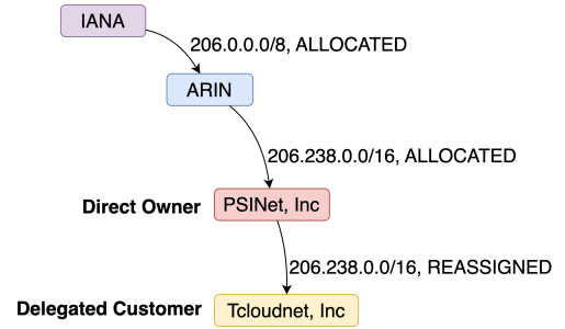
Figure 1: Prefix delegation hierarchy.
