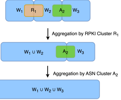
Figure 3: Aggregation of WHOIS prefix clusters via intersecting RPKI prefix clusters & ASN prefix clusters.
