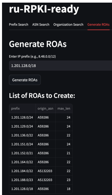
Figure 14: ru-RPKI-ready UI (generating ROA configurations)
