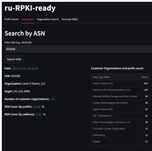
Figure 13: ru-RPKI-ready UI (search results for ASNs)
