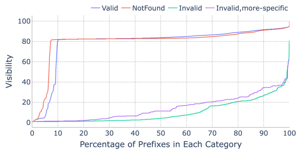
Figure 15: Visibility of routed IPv4 prefixes by RPKI status; RPKI Invalid prefixes have significantly lower visibility; Data: 1 April, 2025
