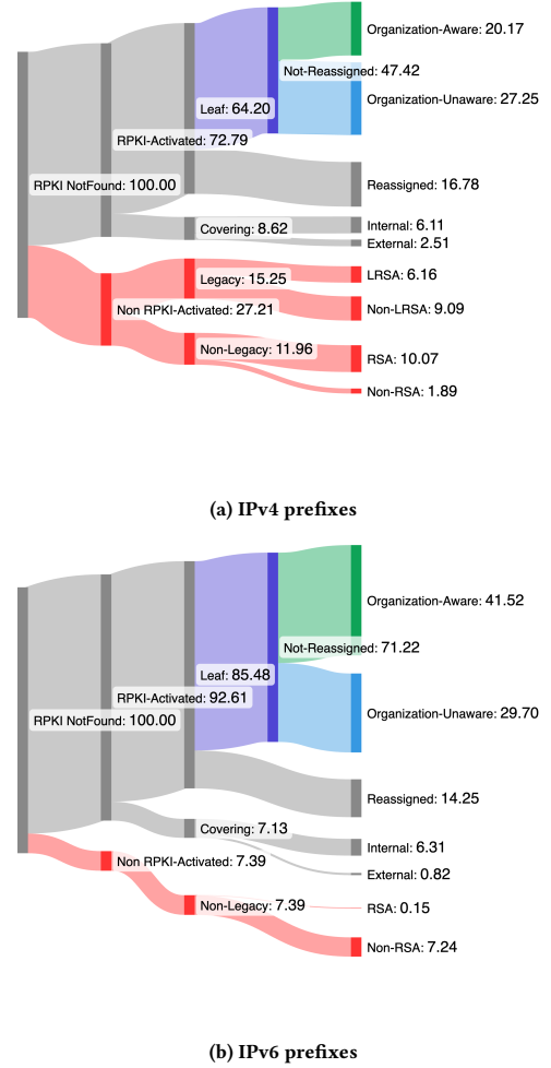
Figure 8: Percentage of routed IPv4 and IPv6 prefixes not covered by ROAs in each category of ru-RPKI-ready; RPKI-Ready prefixes (marked purple) and Low-Hanging prefixes (marked green) have a simpler ROA planning stage in comparison to other categories of prefixes.
