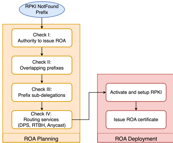
Figure 7: Structured flowchart for ROA planning &amp; deployment
