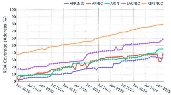
Figure 2: ROA coverage of routed IPv4 address space among the five RIRs; RIPE consistently has the highest adoption among all RIRs
