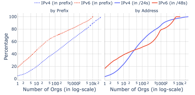
Figure 11: CDF of RPKI-Ready prefixes and addresses by Organization; 10 largest organizations own more than 20% and 40% of the RPKI-Ready IPv4 and IPv6 prefixes respectively
