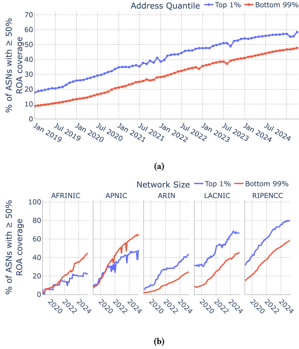
Figure 4: RPKI adoption in Large vs. Small ASes
