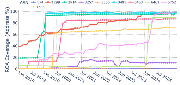
Figure 5: IPv4 RPKI Adoption of Tier-1 ASNs over time
