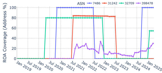
Figure 6: Several networks have issued ROAs for their address space and later dropped them
