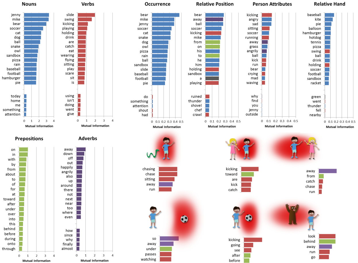
Fig. 7. The words with the highest total MI and CMI scores across all features for different part of speech (left). The words with highest total scores across different features types (top-right). Colors indicate the different parts of speech. Top non-nouns for several relative spatial features using object orientation (bottom-right).
