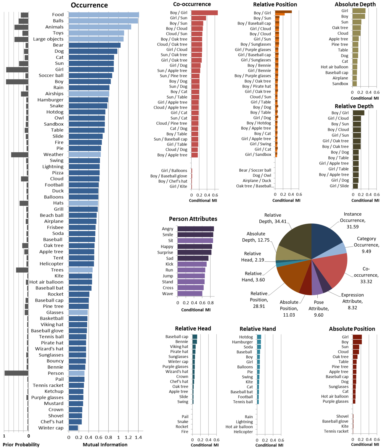
Fig. 5. The mutual information measuring the dependence between classes of semantically similar scenes and the (left) occurrence of objects, (top) co-occurrence, relative depth and position, (middle) person attributes and (bottom) the position relative to the head and hand, and absolute position. Some mutual information scores are conditioned upon other variables (see text.) The pie chart shows the sum of the mutual information or conditional mutual information scores for all features. The probability of occurrence of each piece of clip art occurring is shown to the left.
