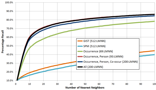
Fig. 6. Retrieval results for various feature types. The retrieval accuracy is measured based on the number of correctly retrieved images given a specified number of nearest neighbors.
