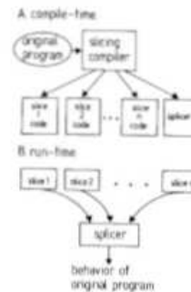
Fig. 5. Parallel execution of slices.
