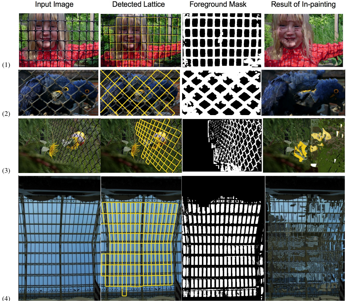
Figure 7. Image de-fencing failed at the inpainting stage.
