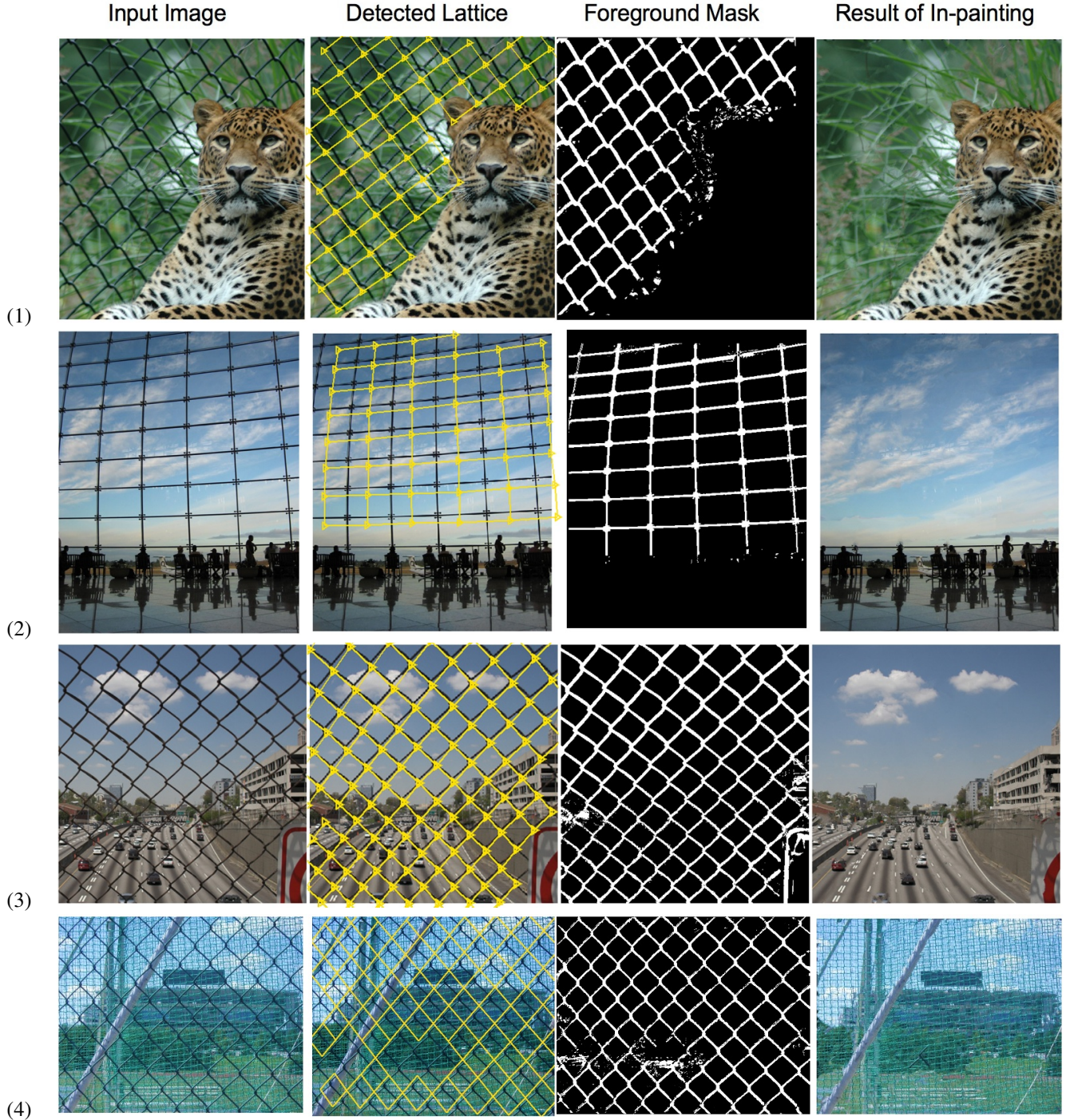
Figure 5. Several relatively promising image de-fencing results demonstrate the effectiveness of the proposed, translation symmetry-based detection-classification-inpainting method.
