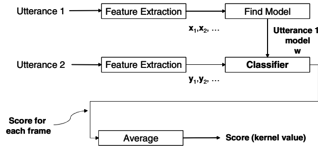
Fig. 3. Sequence kernel.
