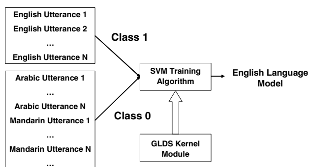
Fig. 2. Training strategy.
