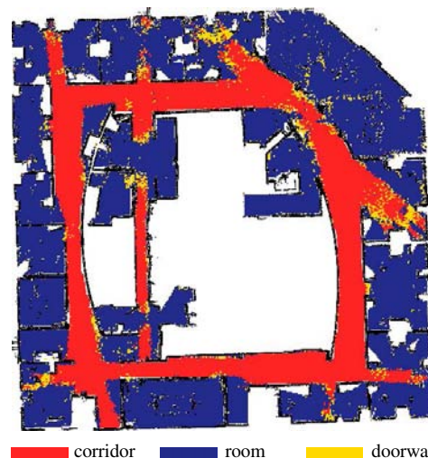
Fig. 8. Classification results obtained by applying the classifier learned for the environment depicted in Figure 1 to the map of the Intel Research Lab in Seattle. The fact that 82.23% of all places could be correctly classified illustrates that resulting classifiers can be applied to so far unknown environments.
