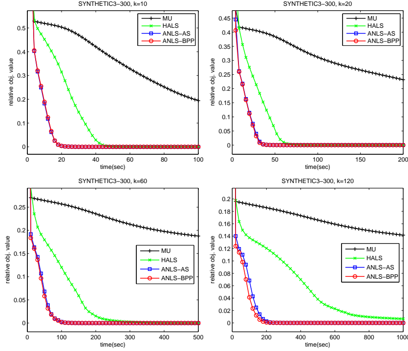
Fig. 1 Relative objective value ( \|\mathcal{X} - [\mathbf{A}^{(1)}, \dots, \mathbf{A}^{(N)}]\|_F / \|\mathcal{X}\|_F ) vs. execution time on the synthetic tensors. Average results of 5 different random initializations are shown. Top row: k = 10 and k = 20 , bottom row: k = 60 and k = 120 .
