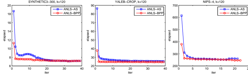
Fig. 3 Execution time of each iteration of the active set (ANLS-AS) and the block principal pivoting method (ANLS-BPP) for k = 120 cases of each data set. Average results of 5 different random initializations are shown. Left: synthetic data set, center: YaleB data set, right: NIPS data set.
