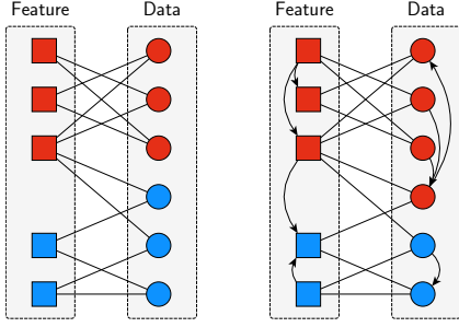
Figure 1: Previous co-clustering model uses undirected bipartite graph (left figure), and our co-clustering model uses bipartite graph combined with directed subgraphs (right figure)
