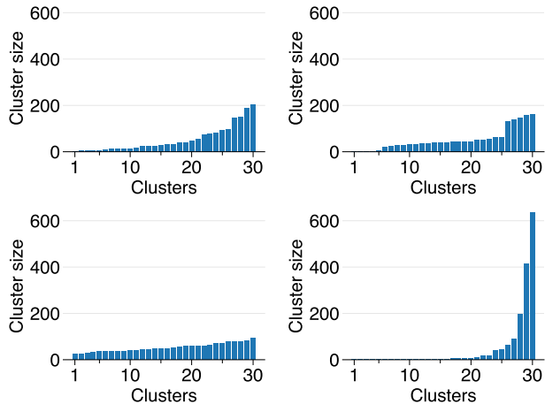
Figure 5: The number of philosophers in 30 co-clusters computed by CoDiNMF (the left upper figure), CoNMF (the right upper figure), LP-FNMTF (the left bottom figure) and SCo (the right bottom figure).
