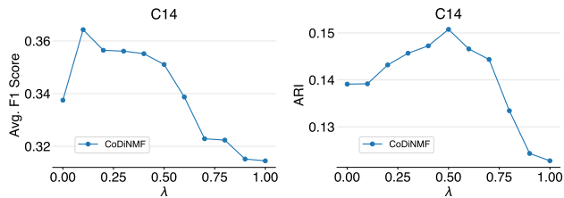
Figure 4: F1 score and ARI of CoDiNMF on C14 patent data set. There are 11 points corresponding to \lambda \in \{0, 0.1, \dots, 1\} .
