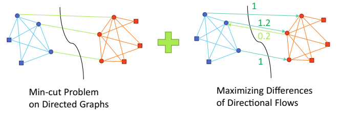
Figure 2: Illustrations of the objective function. Min-cut problem of directed graphs can be derived by considering the sum of all directional cuts between different co-clusters (left figure). An additional term helps to control a net directional flow which is the sum of differences of directional flows (right figure).
