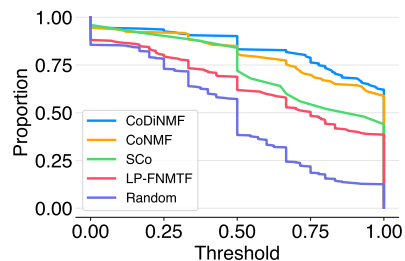
Figure 7: The proportion of cluster pairs of philosophers which are in the upper area above the threshold in Fig 6 is computed and displayed.
