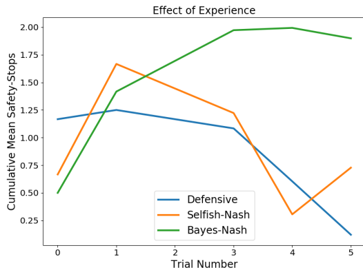
Fig. 8. Effect of experience in the Human-Robot study. It shows the cumulative safety stops for the robot averaged over the trials. For the Defensive and Selfish-Nash conditions, the number of stops decreases with more trials, indicating that the human learns to avoid collision. However, for Bayes-Nash, the safety stops first increase and then remain constant, perhaps due to the difficulty in adapting to an agent whose behavior is not fixed.
