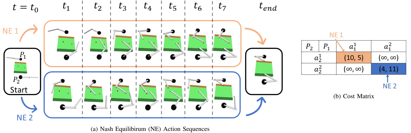
Fig. 1. A scenario where two agents, P_1 and P_2 , move the red and black blocks to their respective goal locations. In (a), we show two sequences of actions starting in the same state at t_0 , and ending in the same goal state at t_{end} . While each action sequence (trajectory) is a Nash Equilibrium (NE), they both favor different agents. NE1 (top) favors P_2 by allowing it to reach its goal first, NE2 (bottom) favors P_1 . A cost function is illustrated in (b), where each cell is a tuple containing the cost of the actions for P_1 and P_2 respectively. Here, our action space has only 2 actions per agent, A_1 = \{a_1^1, a_1^2\} and A_2 = \{a_2^1, a_2^2\} .
