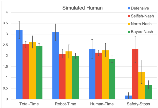
Fig. 4. Results from the experiment involving a simulated human. Note that our proposed approach, Bayes-Nash, is safer than all the non-defensive baselines and similar in task completion time to the Selfish-Nash baseline. Error bars represent standard error of the mean (SEM).
