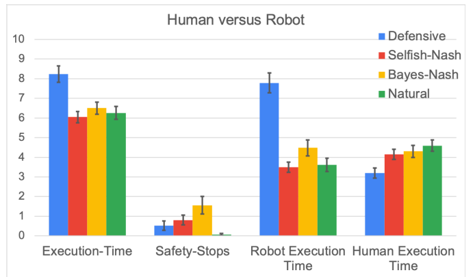
Fig. 7. Human-Robot Study. Defensive and Selfish are baselines, Bayes-Nash is our approach and the Natural agent refers to the human-human study results where the participants acted naturally. Error bars represent SEM.
