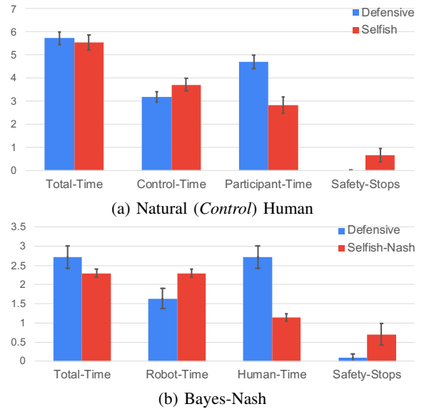
Fig. 5. (a) Plots the interaction task metrics for the naturally acting human in the presence of either a selfish or defensive participant in the human-human study; (b) The same metrics but for the interaction of Bayes-Nash with the Selfish and Defensive baselines. The similarity in the relative trends across (a) and (b) highlight the similarity of Bayes-Nash to a real human agent. Error bars represent SEM.
