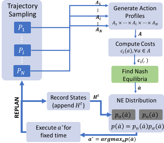
Fig. 3. Framework. We first plan trajectories, then use the cost to compute all Pareto-optimal Nash equilibria, then combine the norm and inferred-personality distributions to select the most likely equilibrium. This action is partially executed before repeating the whole process until the task completes.
