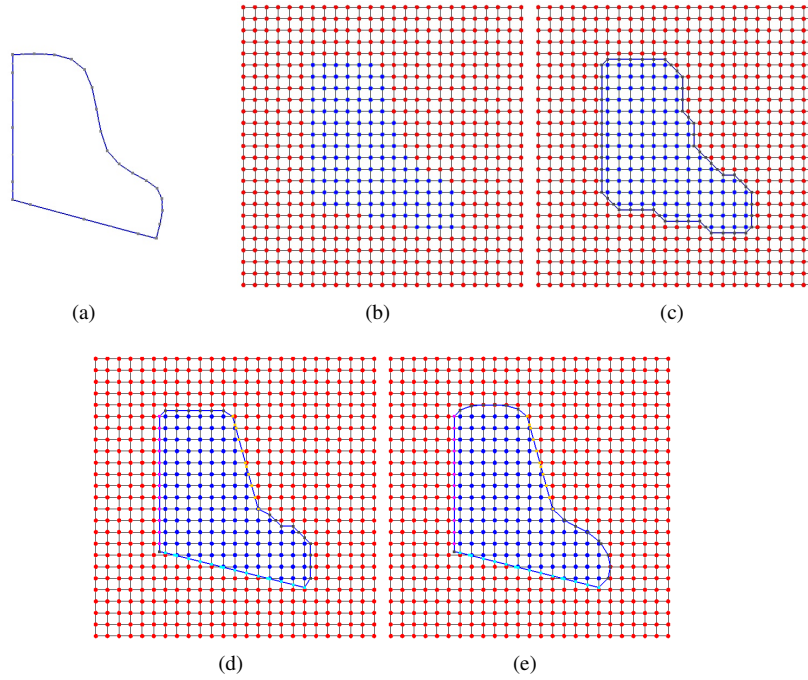
Figure 2: 2D region M bounded by straight and curved edges (a) Red/blue classification of grid-samples produced by rasterizing M . (b) Reconstructed isocontour S with vertices at stick midpoints. (c) Straight edges are recovered by snapping the vertices of each cluster to its flat. (d) A pressed version S' of S is obtained after 50 pressing iterations. (e) Its straight and curved edges correspond to those of M .
