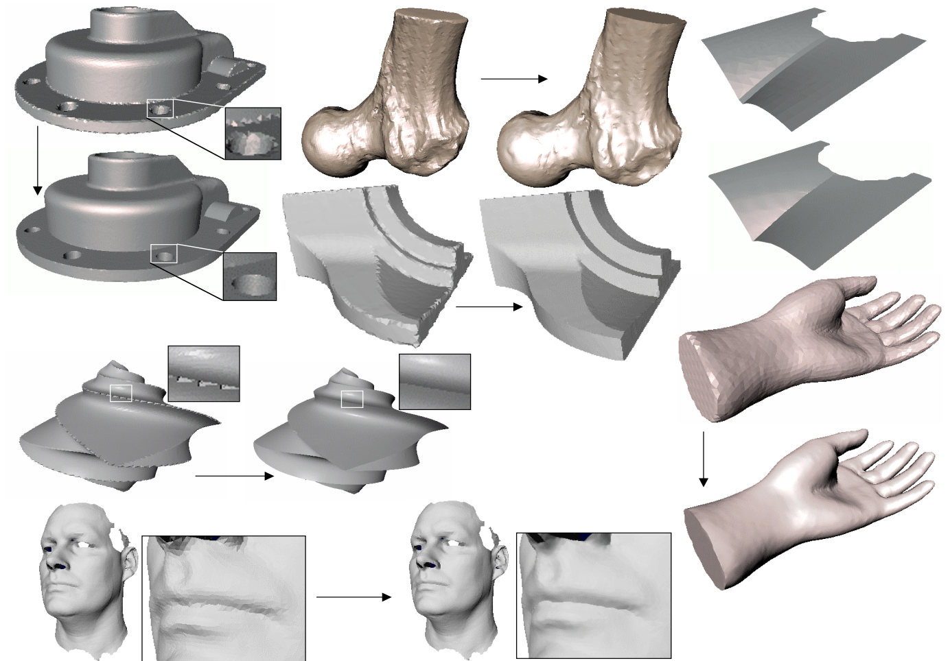
Fig. 18: Some examples of models improved through Sharpen&Bend. Corresponding numerical results are reported in Fig. 14.
