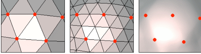
Fig. 10: Butterfly subdivision: an example showing how an initial triangle mesh (on the left) is refined by a subdivision step (middle). On the right, the limit surface is shown. The red dots indicate the vertices of the initial triangle mesh, whose coordinates are not modified by the subdivision process.
