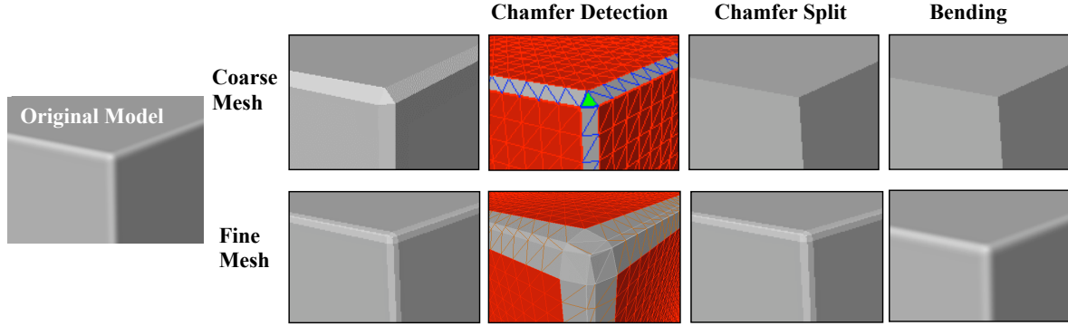
Fig. 17: Unwanted creases may be produced if an original surface has blends whose radius is smaller than the inter-sample spacing (top row). If the sampling step is small compared to the blend radius, the blends are not modified by Edge-Sharpener (bottom row), while they are smoothed as expected by Bender.
