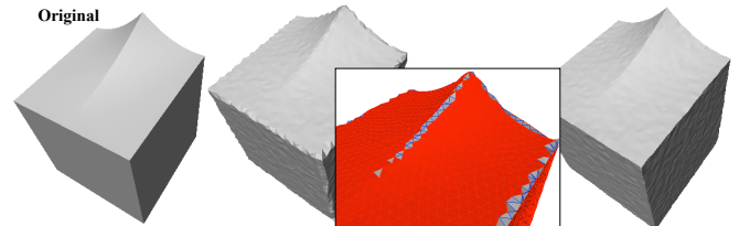
Fig. 16: Reconstruction of a sharp feature which blends smoothly onto a flat surface. The "ripple" of the strip of chamfer triangles prevented the red region to expand on the chamfer.
