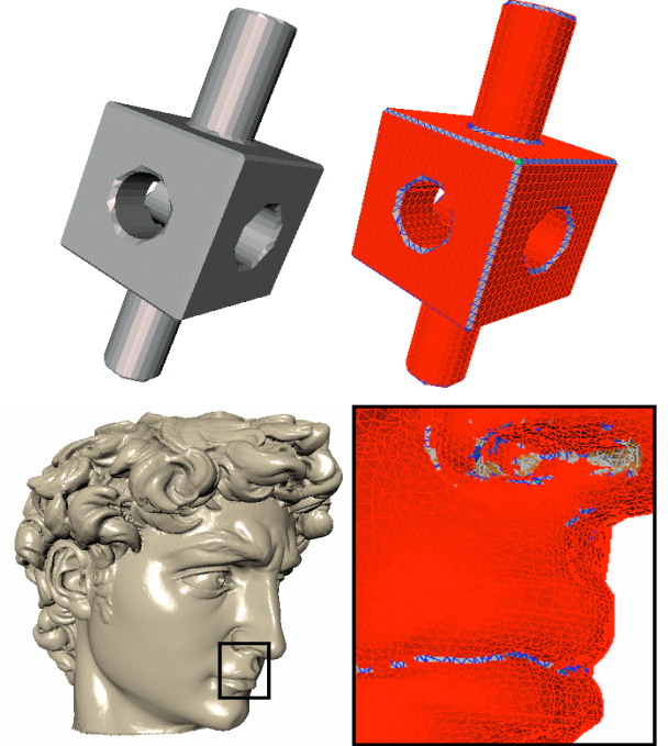
Fig. 3: Chamfers identified by Edge-Sharpener on a Marching-Cubes generated model (top row) and on the simplified version of a laser scanned model of Michelangelo's David (bottom row). Some edges are still gray or brown.
