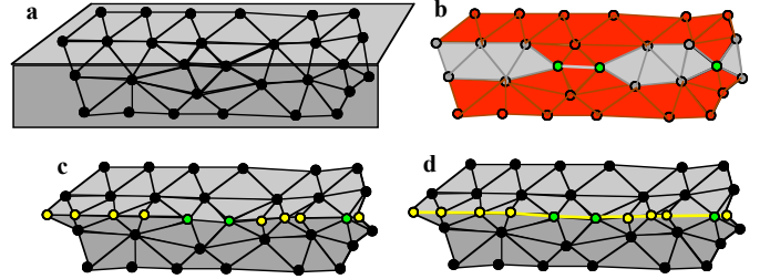
Fig. 9: An original surface with a sharp edge is approximated by the triangulation of a feature-insensitive sampling [a]. Filter 3bis has detected a non-brown edge having two incident red triangles and has tagged its vertices. Filter 3bis has also tagged a vertex having a non manifold red neighborhood (tagged vertices are shown in green in [b]). After the subdivision of the chamfer triangles, all of the newly inserted vertices have been tagged (yellow vertices in [c]). Finally, all of the edges joining two tagged vertices have been tagged as sharp (yellow edges in [d]). Note that the vertices of the tagged edges may have been tagged either in [b] or in [c].
