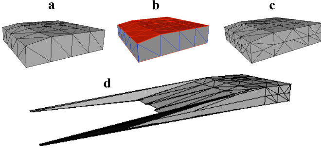
Fig. 7: In an input model (a) the chamfer edges joining nearly parallel surfaces (b) were subdivided without moving the new vertices (c). A wrong model (d) would be obtained without our edge-length check.
