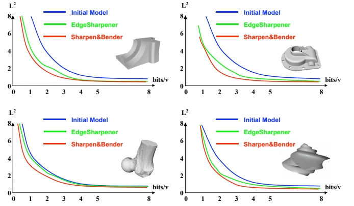
Fig. 15: Impact of EdgeSharpener and Bender on the rate-distortion curves of the SwingWrapper compressor. Bit-per-vertex rates are relative to the # of vertices of the original model. Errors are expressed in units of 10^{-4} of the bounding-box diagonal.
