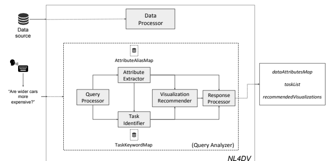
Figure 2: NL4DV architecture
