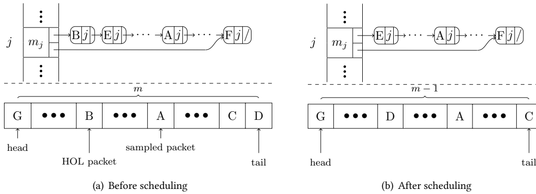
Fig. 2. Illustrating the action of the QPS data structures on a single input port.
