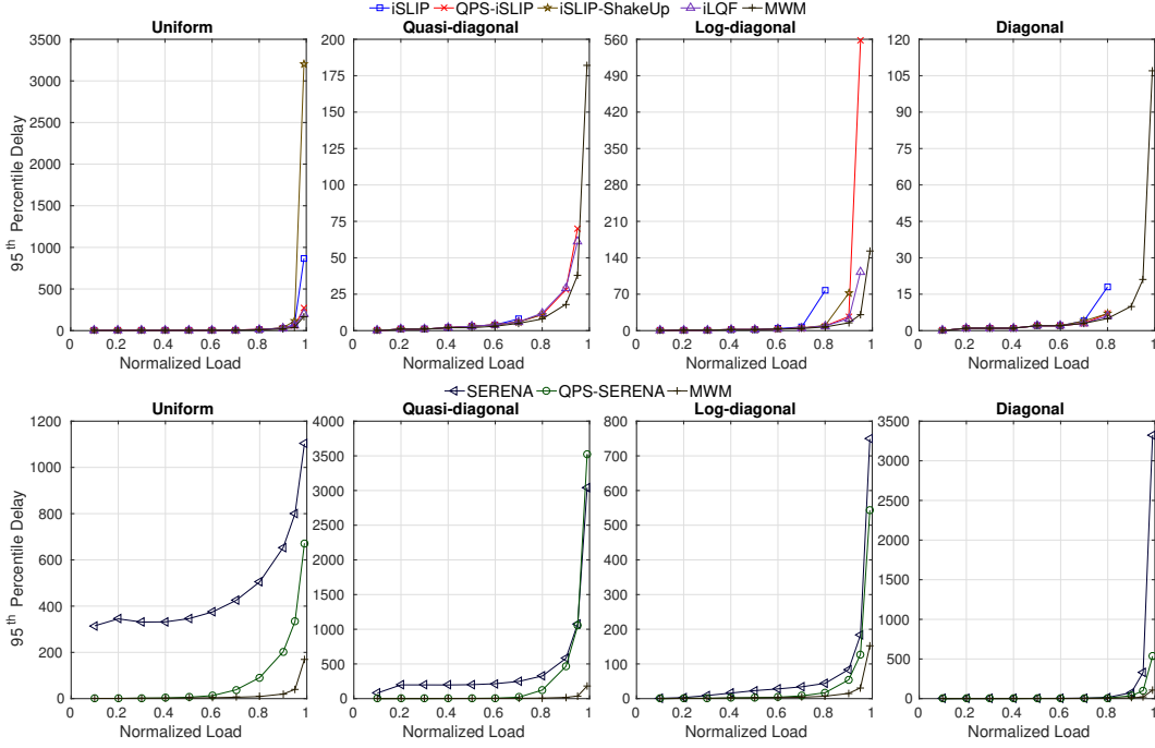
Fig. 4. 95 th percentile delay under Bernoulli i.i.d. traffic arrivals with the 4 load matrices.
