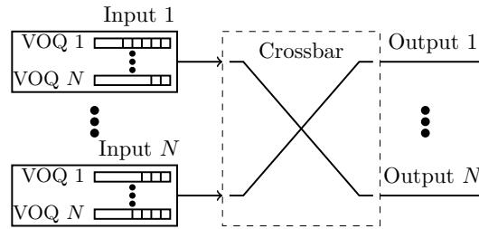
Fig. 1. Generic input-queued crossbar switch.
