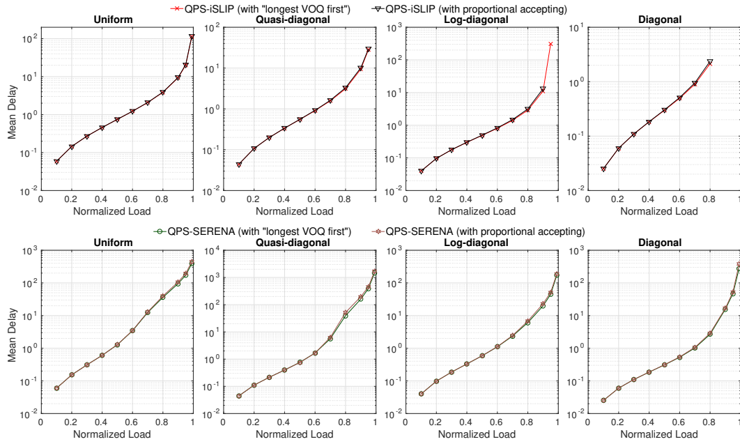
Fig. 8. Mean delays for QPS-iSLIP and QPS-SERENA with the 2 different accepting strategies under Bernoulli i.i.d. traffic arrivals with the 4 load matrices.
