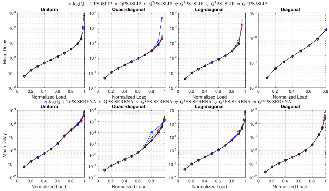
Fig. 6. Mean delays for different FQPS-iSLIP and FQPS-SERENA under Bernoulli i.i.d. traffic arrivals with the 4 load matrices.
