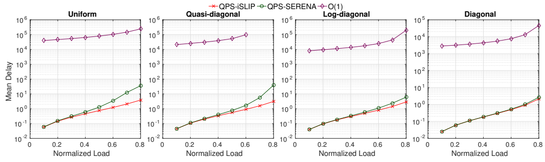
Fig. 10. Mean delay for QPS-iSLIP/QPS-SERENA against O(1) algorithm in [38] under Bernoulli i.i.d. traffic arrivals with the 4 load matrices.
