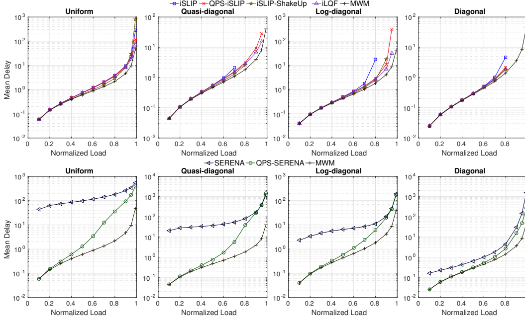
Fig. 3. Mean delays under Bernoulli i.i.d. traffic arrivals with the 4 load matrices.
