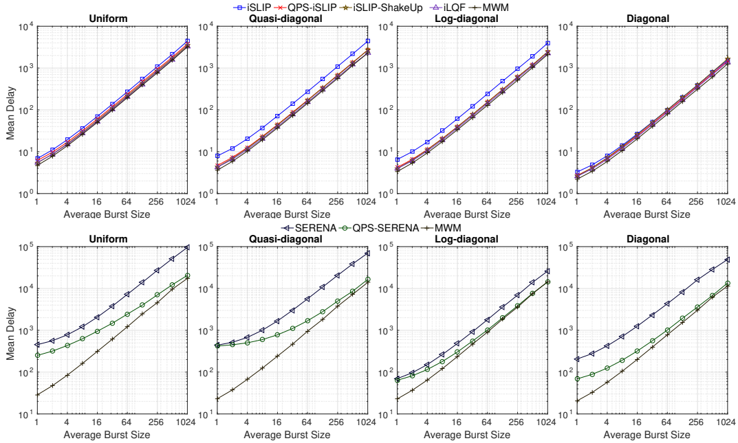
Fig. 5. Mean delays under bursty traffic with the 4 load matrices.
