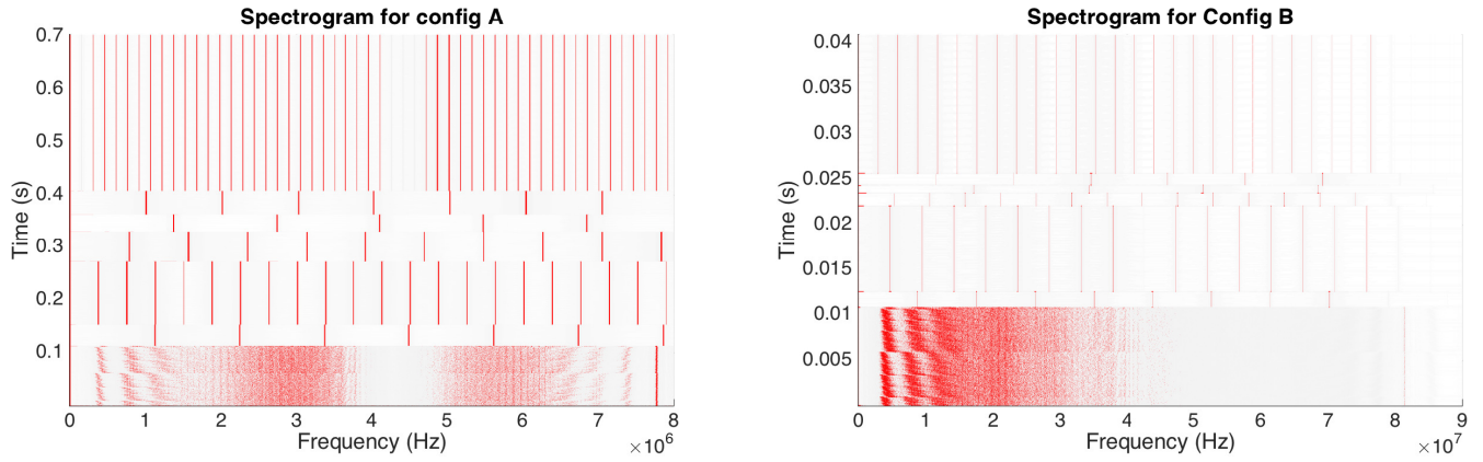
Fig. 8. Spectrograms from two different system configurations for Bitcnt benchmark for large size input.
