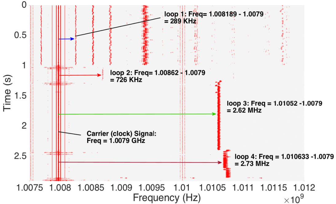
Fig. 3. Spectrogram for Basicmath benchmark with large (profiling run) inputs.
