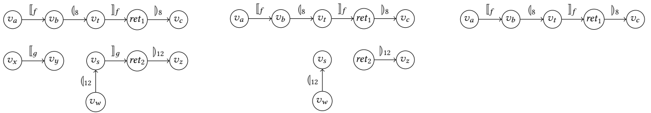
(a) Graph G_1 after the first iteration. The field-write edge v_x \xrightarrow{\llbracket g \rrbracket} v_a , the field-read edge v_c \xrightarrow{\llbracket h \rrbracket} v_z , the call edge v_y \xrightarrow{\langle 11 \rangle} v_s have been eliminated.
