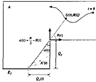
Fig. 3. Base case for a continuous sensing robot
