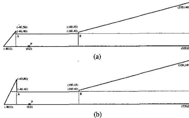
Fig. 7. Two similar polygonal environments
