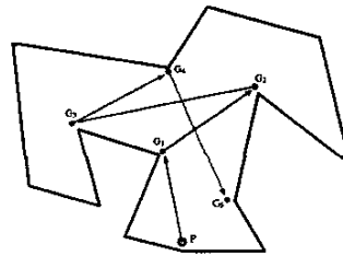
Fig. 9. A simple polygon with non-convex vertices as guards
