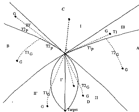
Fig. 10. Optimal paths for the case in which velocity vectors from P are allowed in regions C and D but forbidden in regions A and B
