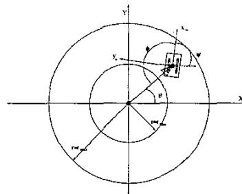
Fig. 1. Coordinate frame assignments for a differential drive robot with camera.
