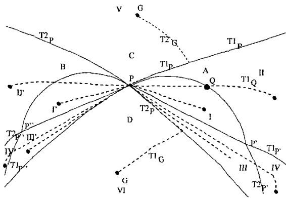
Fig. 8. Optimal paths for the case in which velocity vectors from P are allowed in regions A and B but forbidden in regions C and D
